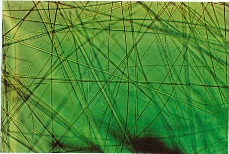
Figure 5. These amphibole fibers, which Dr. Gübelin believed were tremolite, are characteristic of emeralds from Sandawana, Zimbabwe. Photomicrograph by Edward J. Gübelin, magnified 20x, from the Photoatlas of Gemstone Inclusions (1986); used with permission from Opinio Verlag , Basel, Switzerland.
